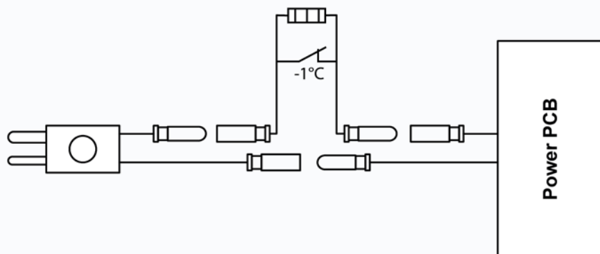
Figure 20 - Wiring diagram for the heaters
