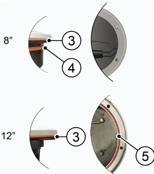
Figure 21 - Fixture gaskets
