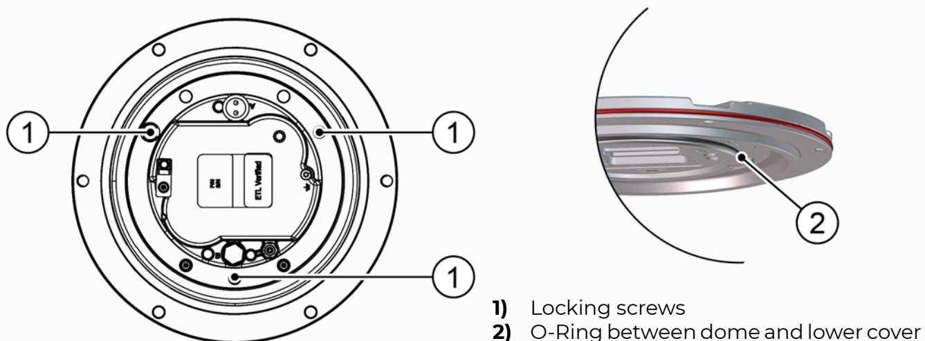
Figure 13 - Lower cover fixing screws (dia. 12)
