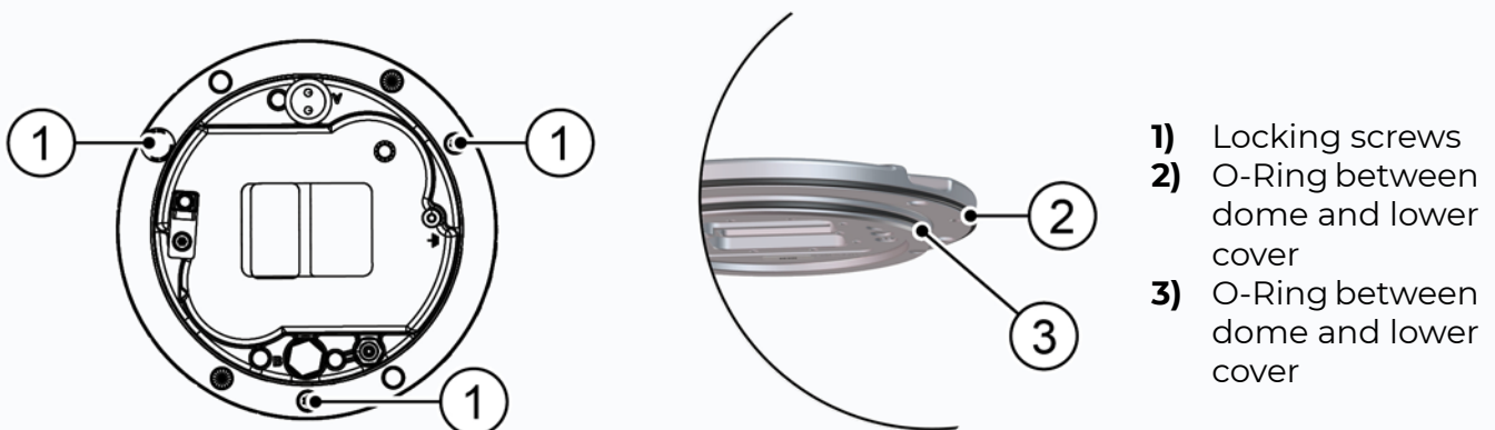
Figure 12 - Lower cover fixing screws (dia. 08)
