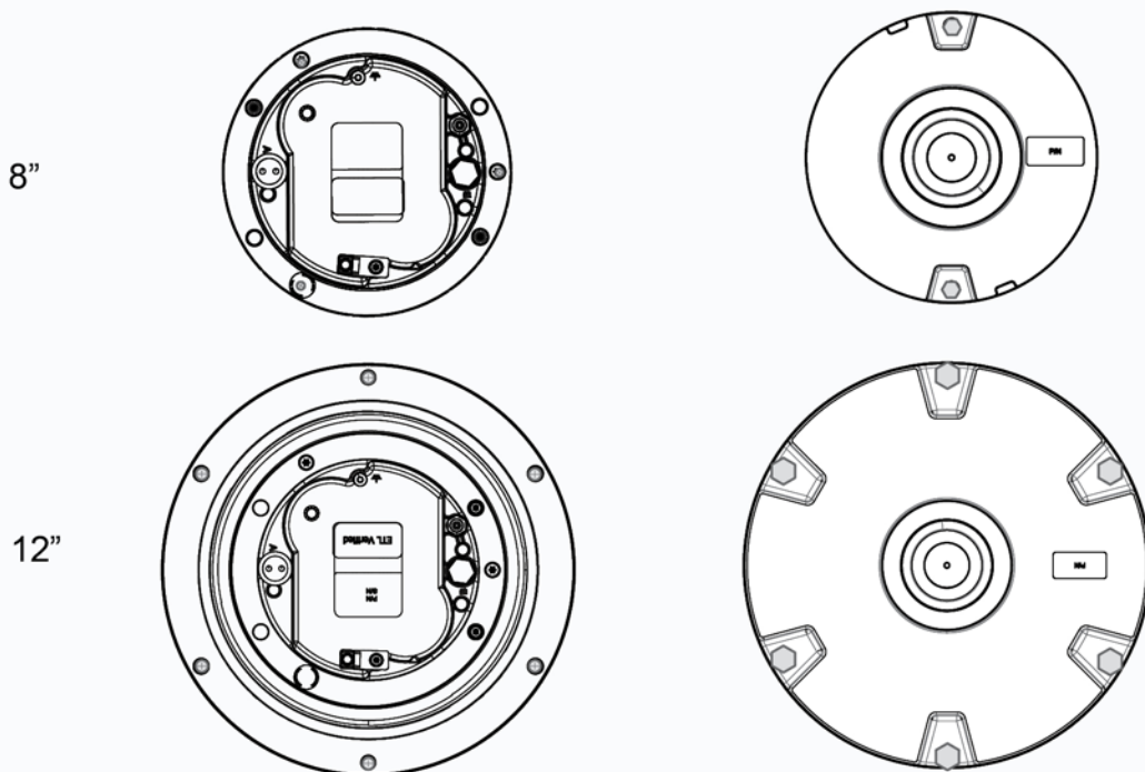
Figure 23 - Tightening elements
