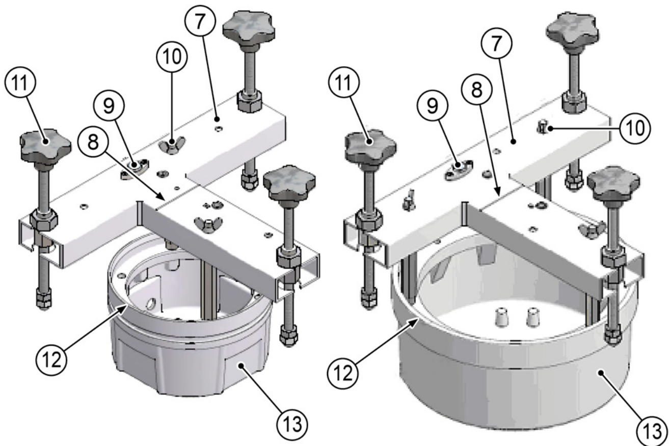
Figure 15 - Shallow base installation details (8" on the left, 12" on the right)
