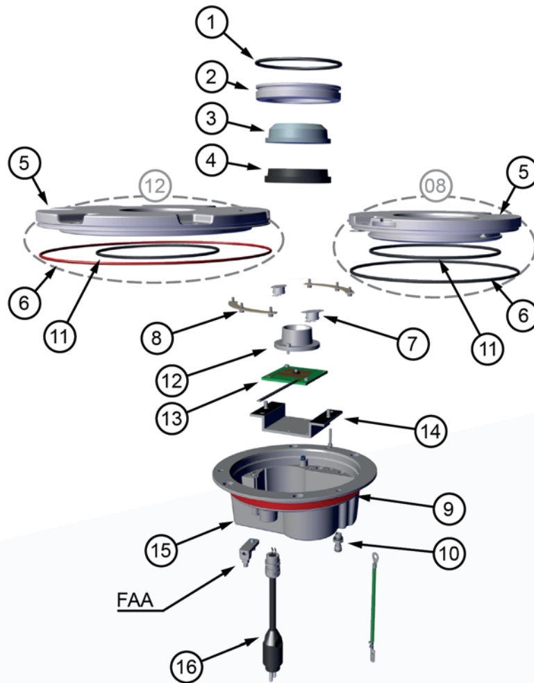
Figure 2 - Exploded view
