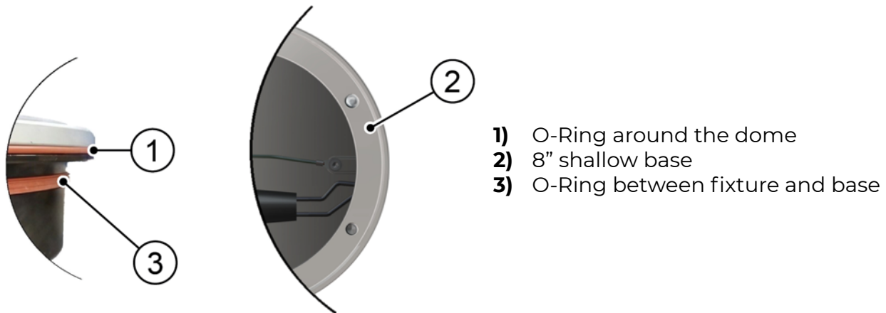
Figure 11 - Gasket for 8" shallow base
