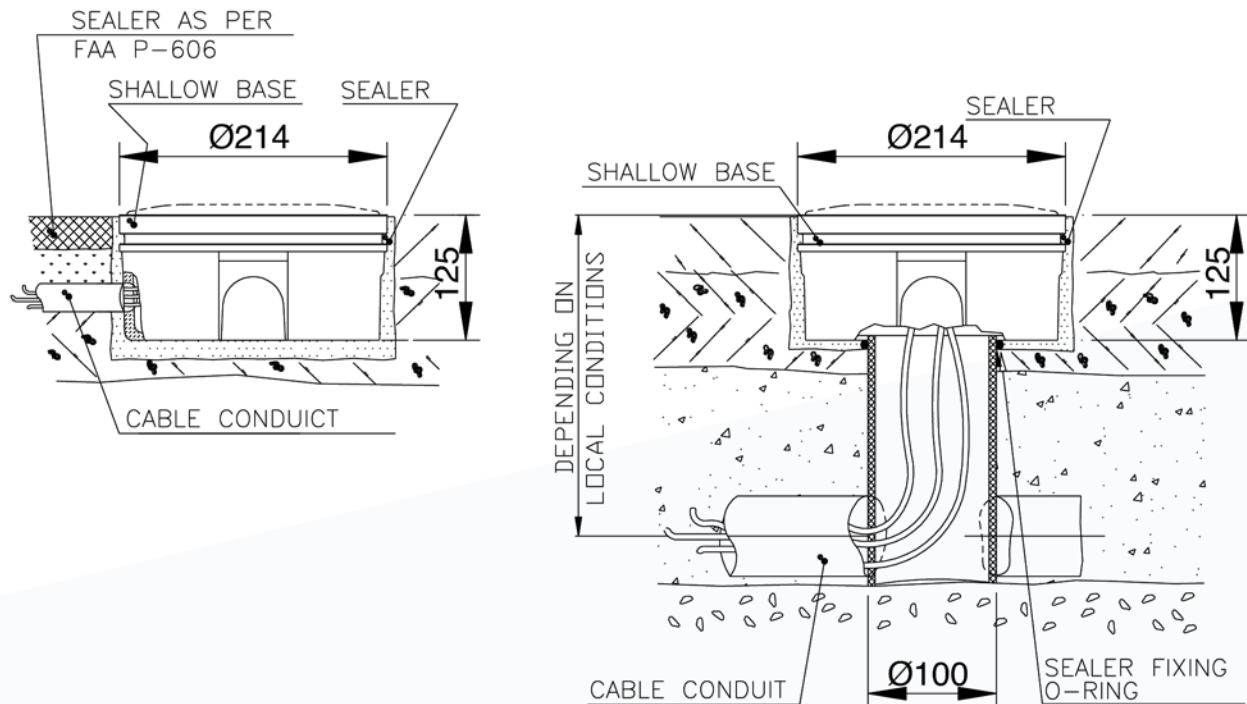
Figure 12 - 8" shallow base for side or bottom ducts (Method "B")
