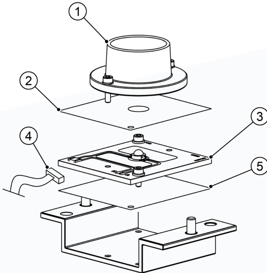
Figure 19 - LED module replacement
