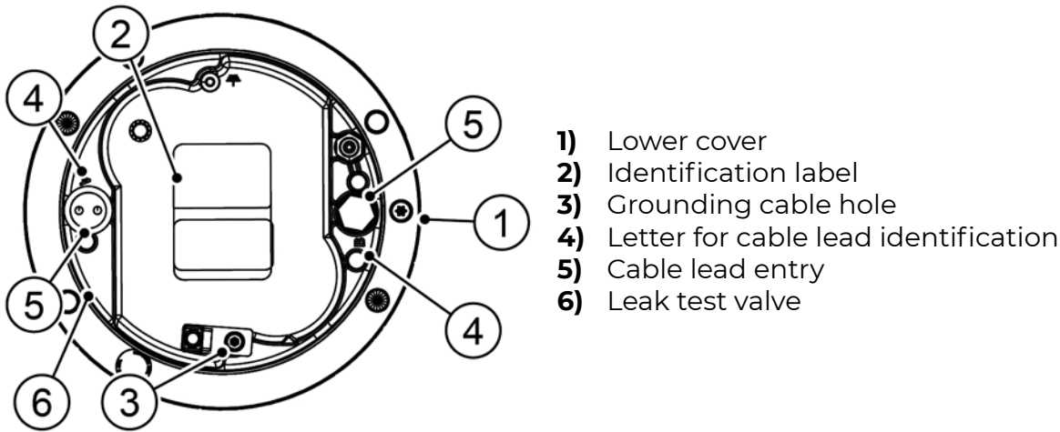
Figure 8 - 8" Lower cover (outside view)
