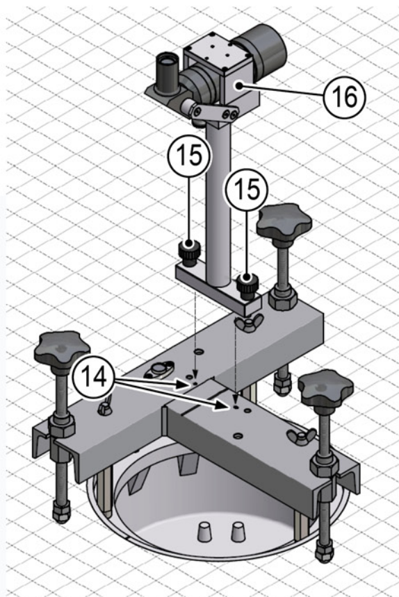
Figure 16 - Optical device (refer to the dedicated manual for further information)
