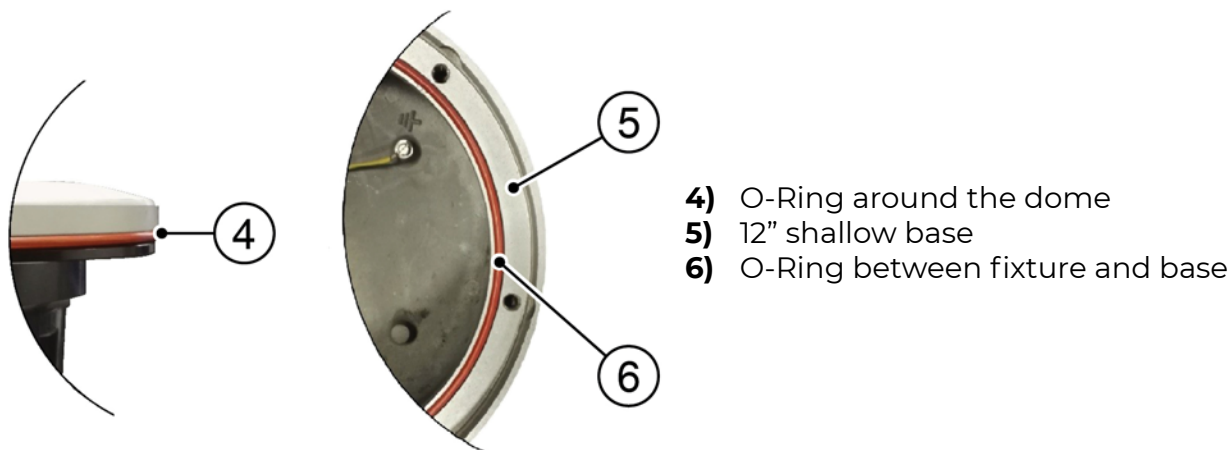
Figure 13 - Gasket for 12" shallow base
