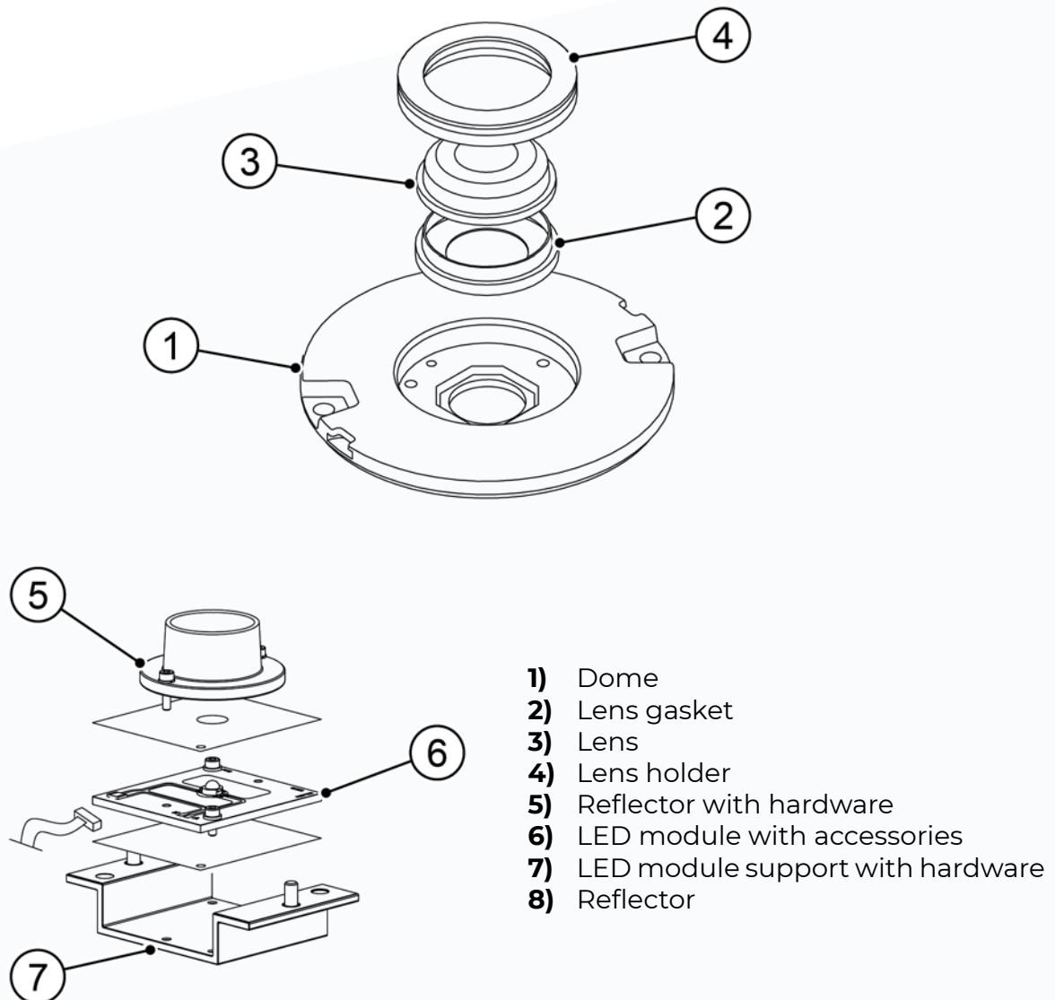
Figure 5 - Optical assembly
