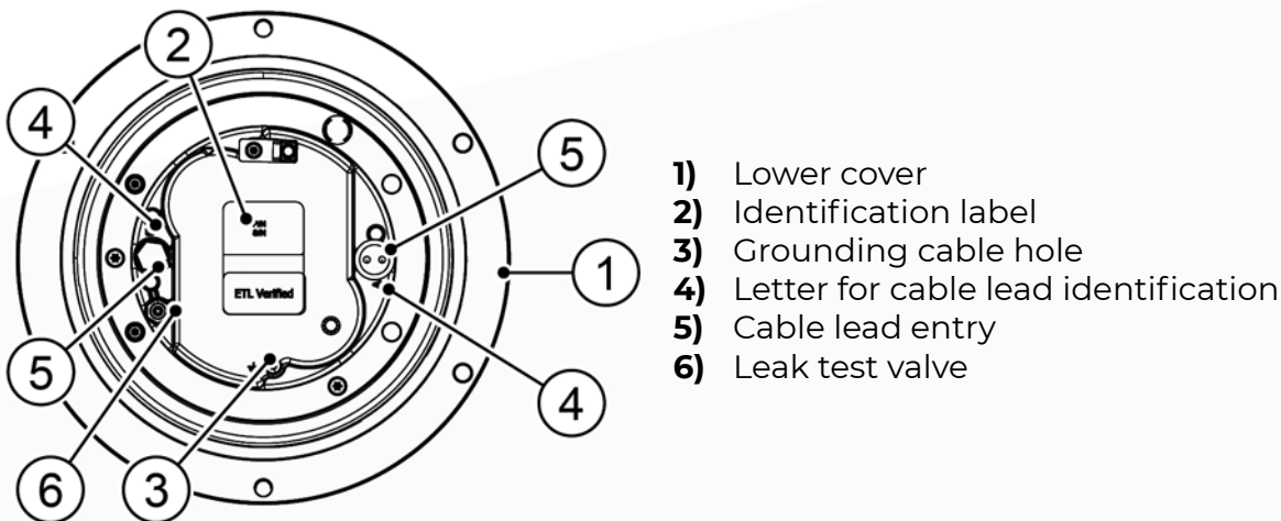
Figure 9 - 12" Lower cover (outside view)
