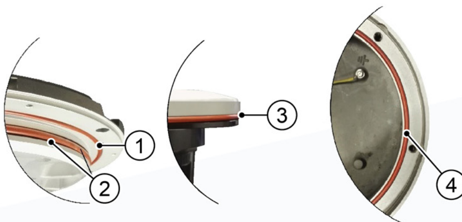
Figure 22 - Fixture gasket
