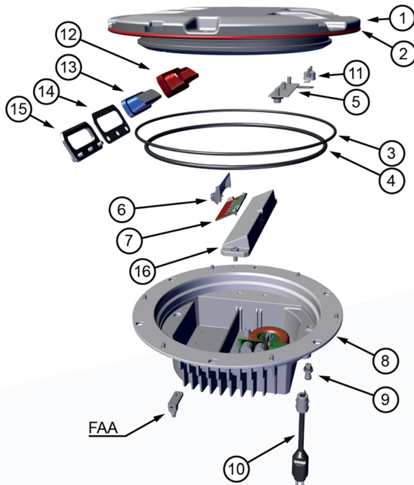
Figure 3 - Exploded view
