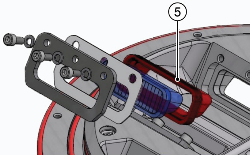
Figure 23 - Prism replacement
