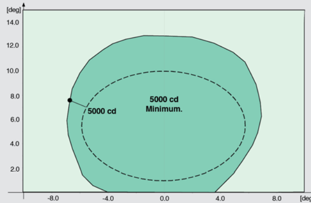
Figure 2 - FAA L-850E Threshold (GREEN)
