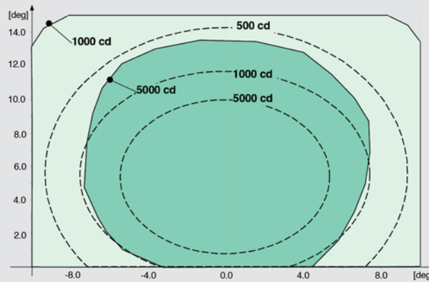
Figure 1 - ICAO Threshold A2-3 (GREEN)
