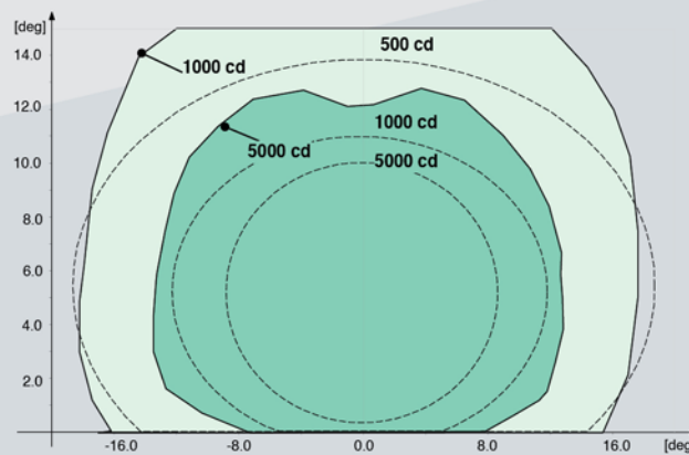
Figure 3 - ICAO Threshold Wing Bar A2-4 (GREEN)
