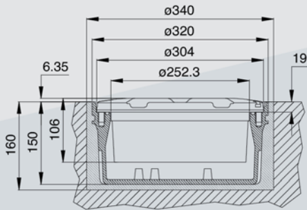
Figure 5 - Shallow base 12" dia.
