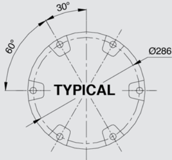
Figure 4 - Light fixture 12" dia.
