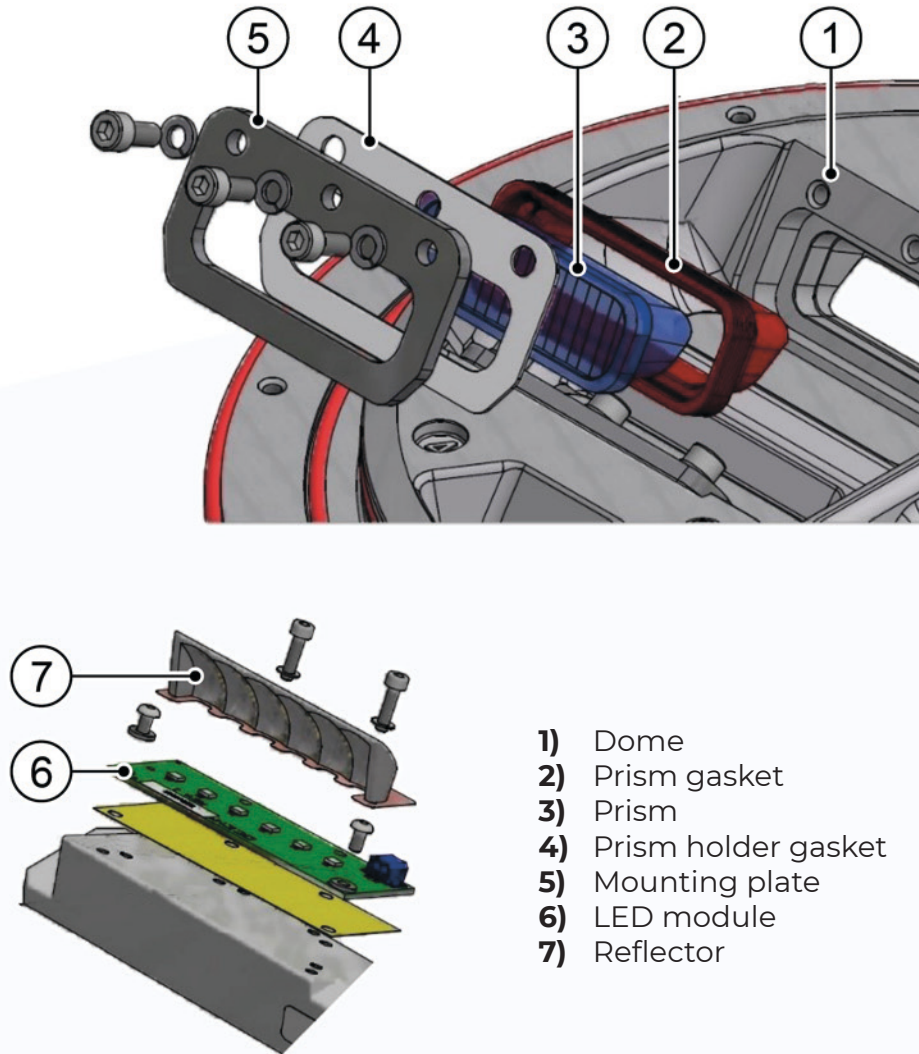
Figure 5 - Optical assembly
