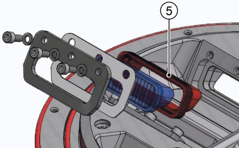
Figure 23 - Prism replacement
