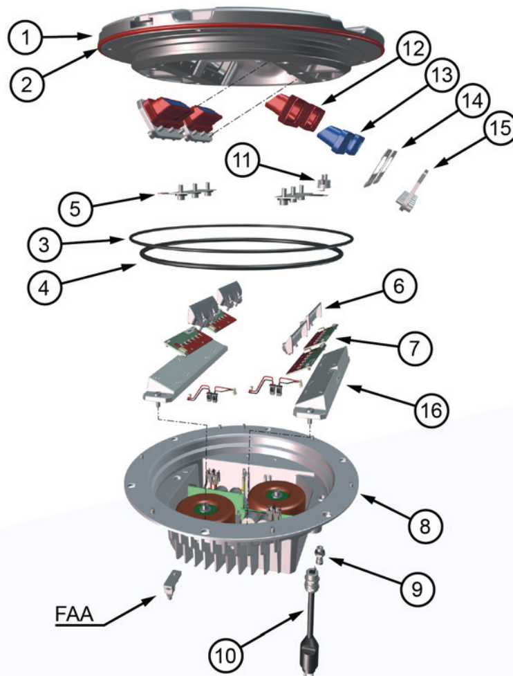
Figure 3 - Exploded view
