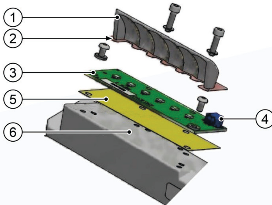
Figure 20 - LED module replacement
