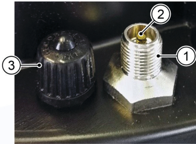
Figure 26 - Lower cover with pressure valve
