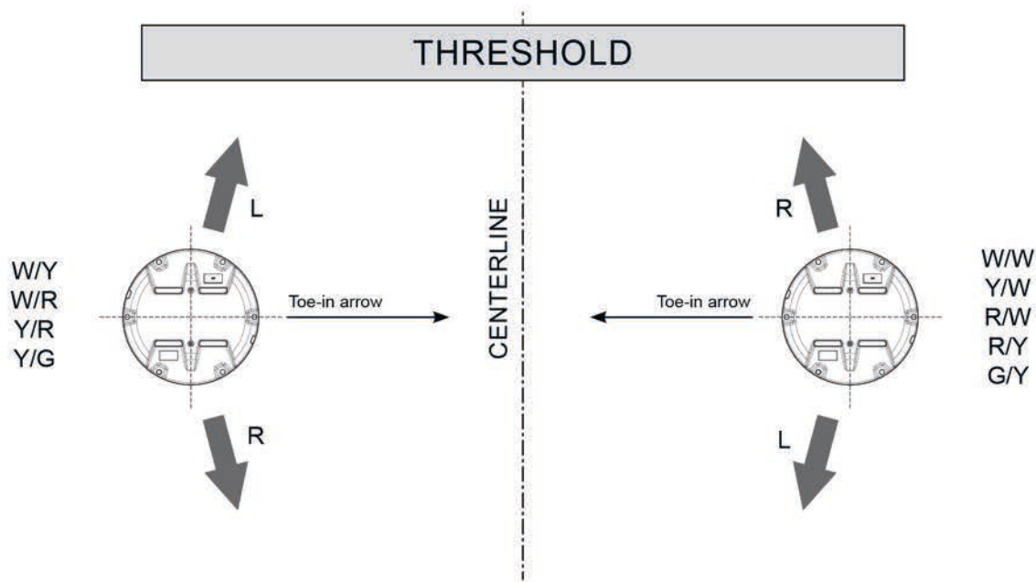
Figure 2 - Toe-in of the fixtures
