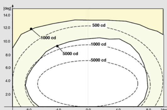
Figure 2 - ICAO A2-10 60 m - White
