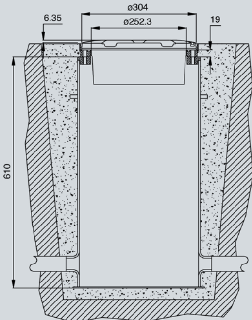
Figure 8 - L-868 Deep base 12" dia.
