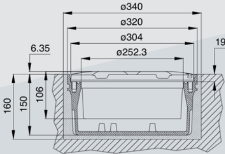
Figure 7 - Shallow base 12" dia.
