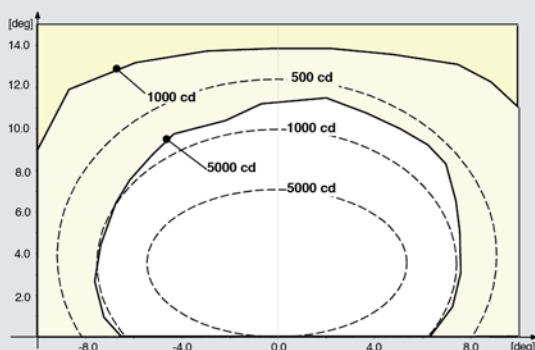
Figure 1 - ICAO A2-9 45 m - White
