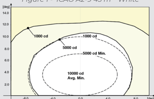
Figure 3 - FAA L-850C - White
