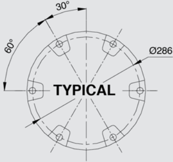
Figure 6 - Light fixture 12" dia.
