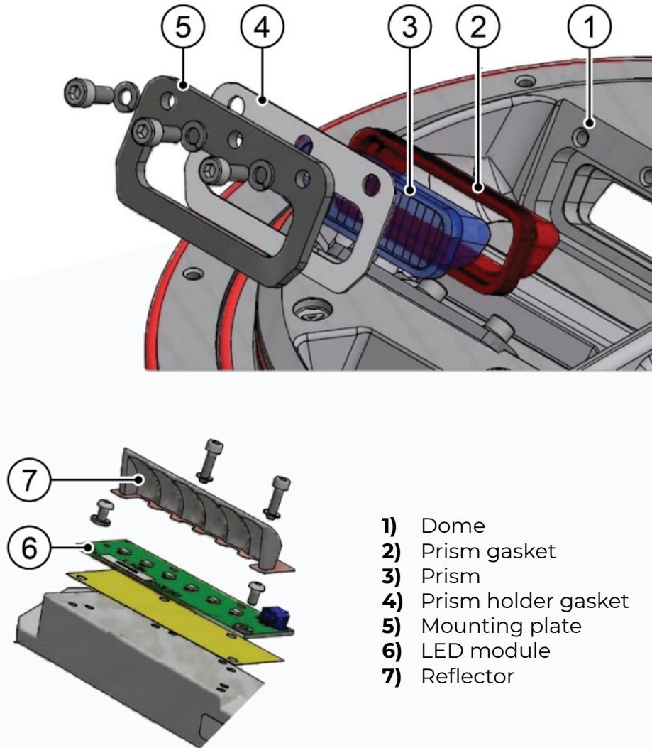
Figure 4 - Optical assembly
