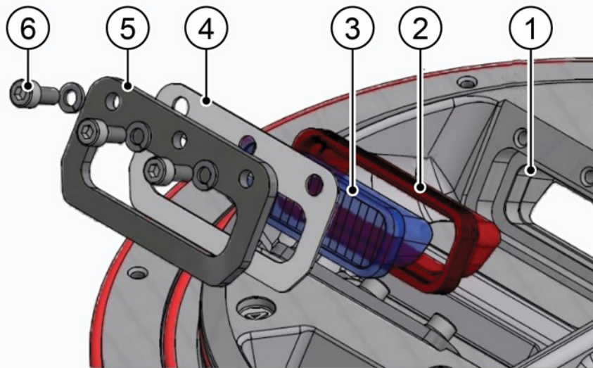
Figure 21 - Prism replacement
