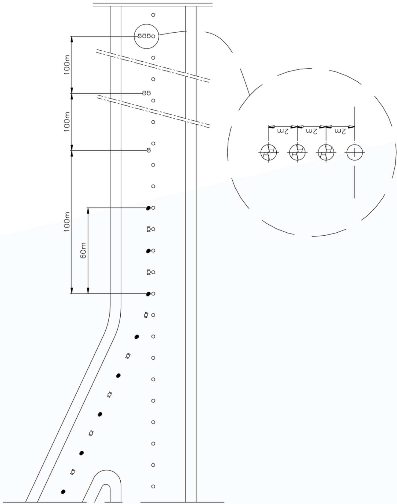
Figure 11 - Example of light unit configuration (R.E.T.I.L.)
