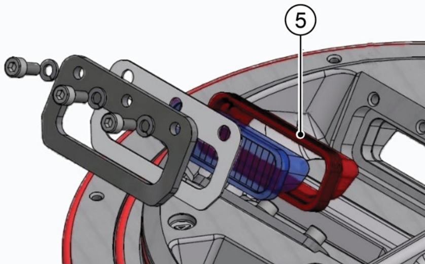
Figure 25 - Prism replacement
