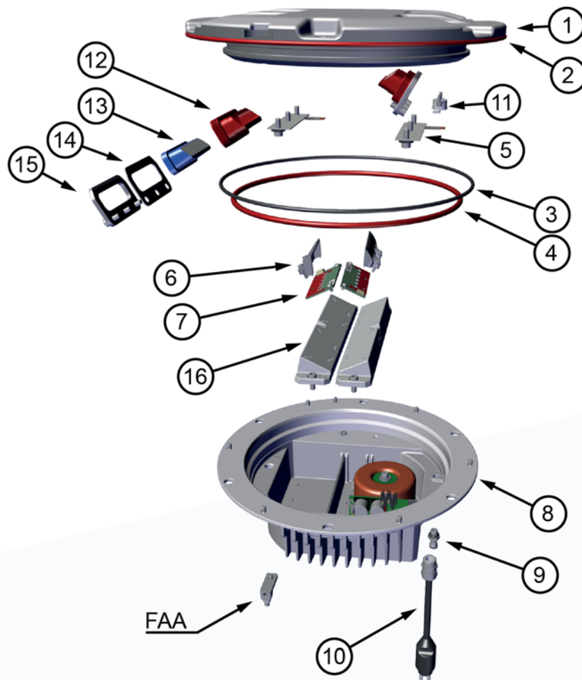
Figure 2 - Exploded view
