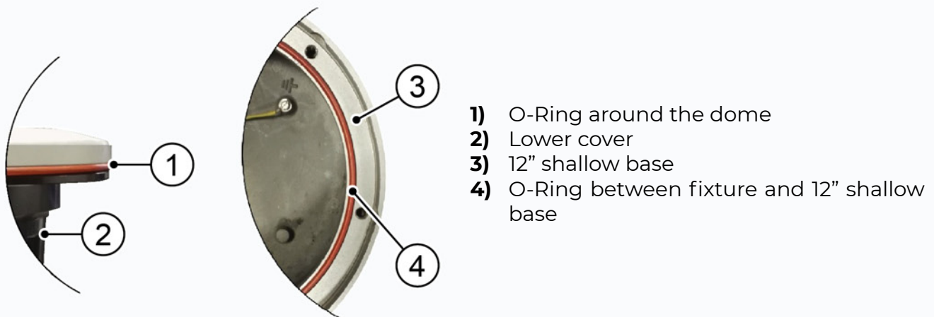
Figure 19 - Fixture gasket
