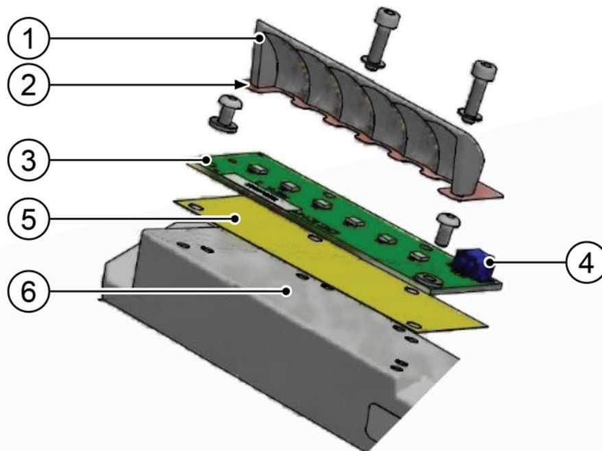
Figure 22 - LED module replacement
