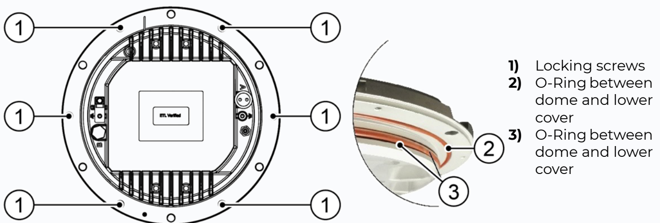
Figure 17 - Lower cover fixing screws
