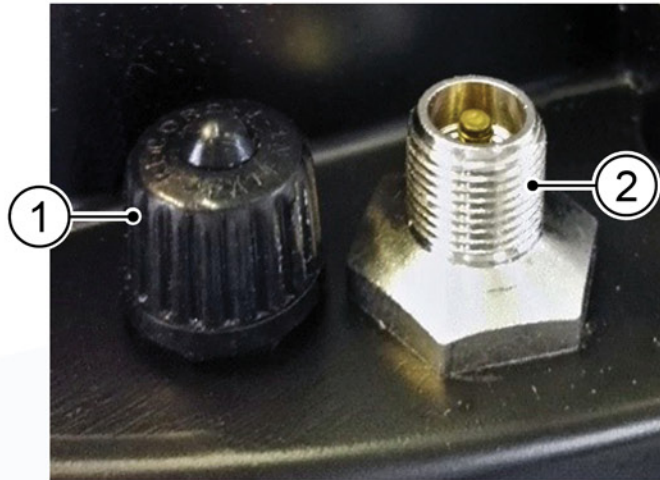
Figure 18 - Lower cover with pressure valve
