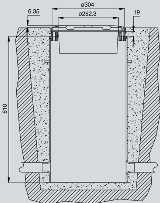
Figure 9 - L-868 Deep base 12" dia.
