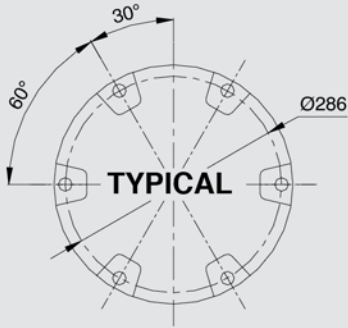
Figure 7 - Light fixture 12" dia.
