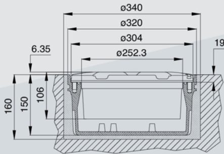
Figure 8 - Shallow base 12" dia.
