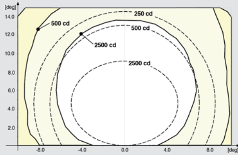
Figure 1 - ICAO A2-7 15 m - White
