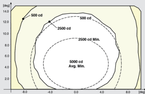
Figure 3 - FAA L-850A - White
