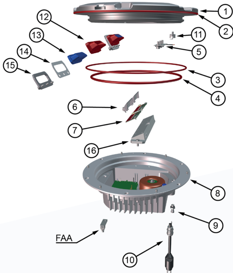
Figure 2 - Exploded view
