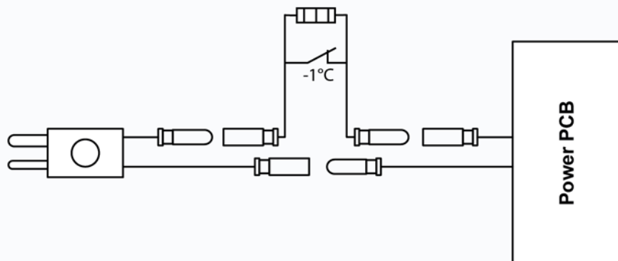
Figure 20 - Wiring diagram for the heaters
