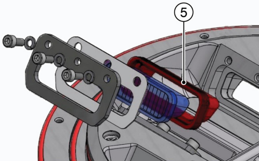
Figure 22 - Prism replacement
