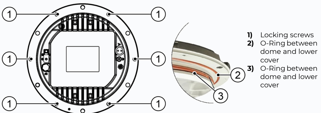
Figure 14 - Lower cover fixing screws
