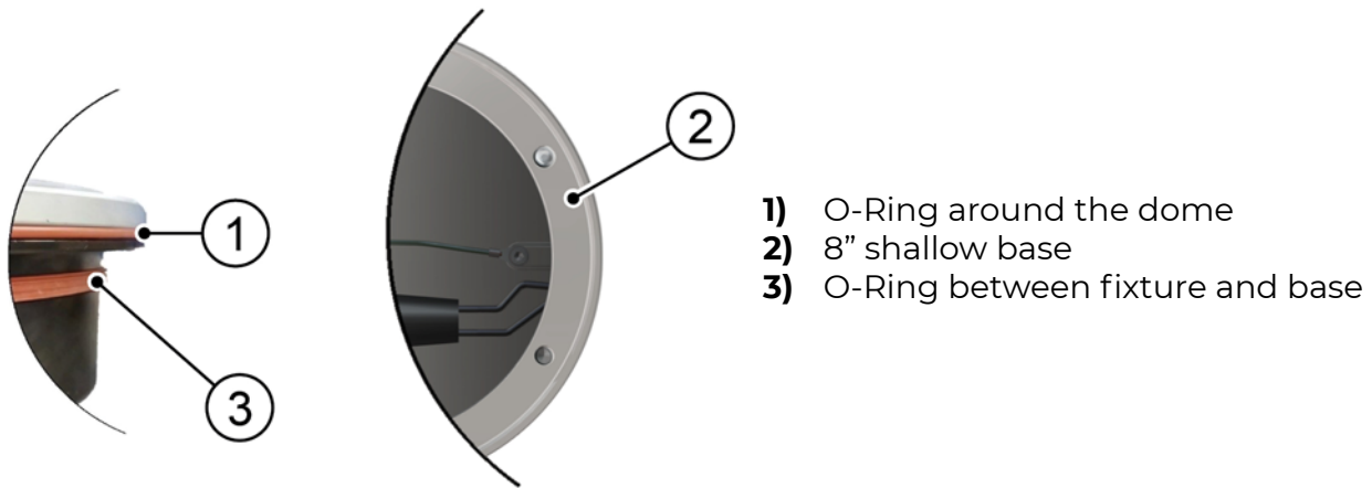
Figure 10 - Gasket for 8" shallow base
