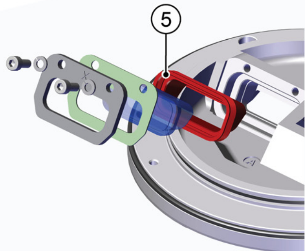
Figure 22 - Prism gaskets
