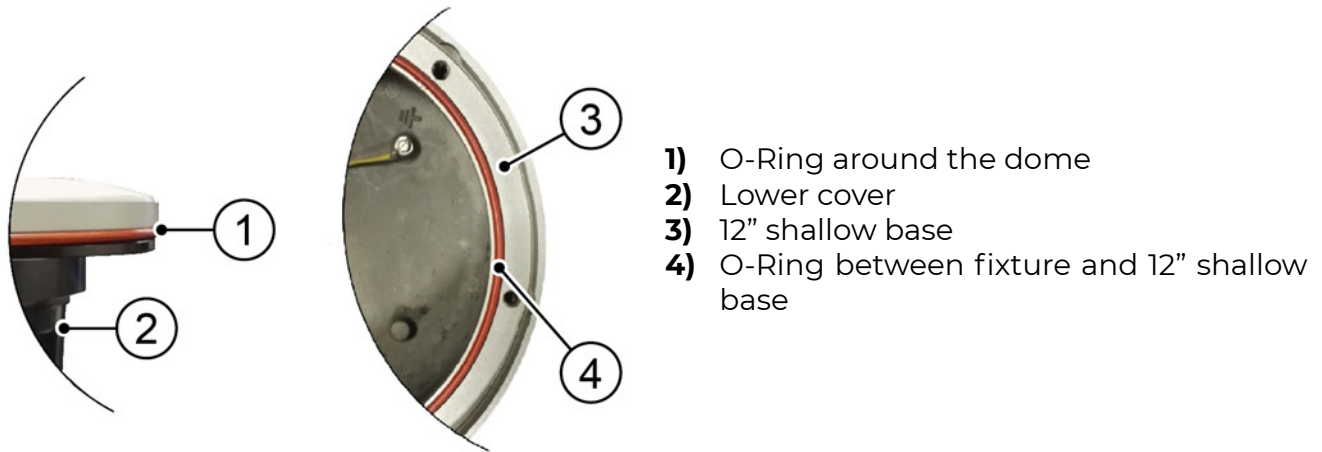
Figure 16 - Fixture gasket dia. 12
