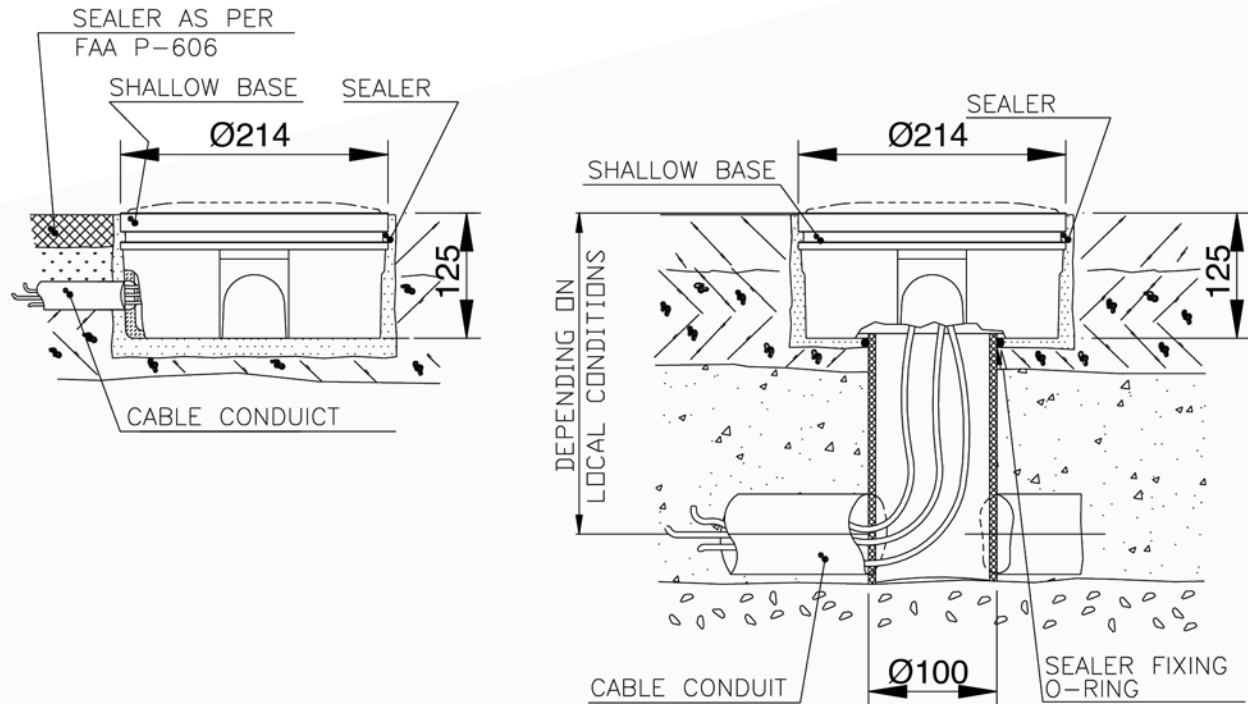
Figure 11 - 8" shallow base for side or bottom ducts (Method "B")
