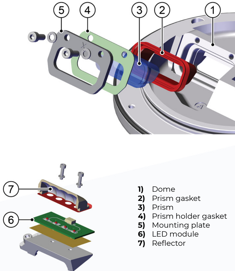
Figure 3 - Optical assembly
