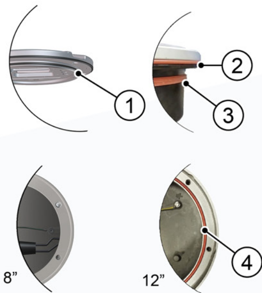
Figure 21 - Fixture gaskets
