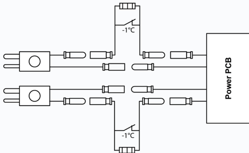
12" Bidirectional Light fixture with 2 power input
