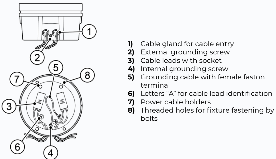
Figure 7 - Lower cover (inside view)
