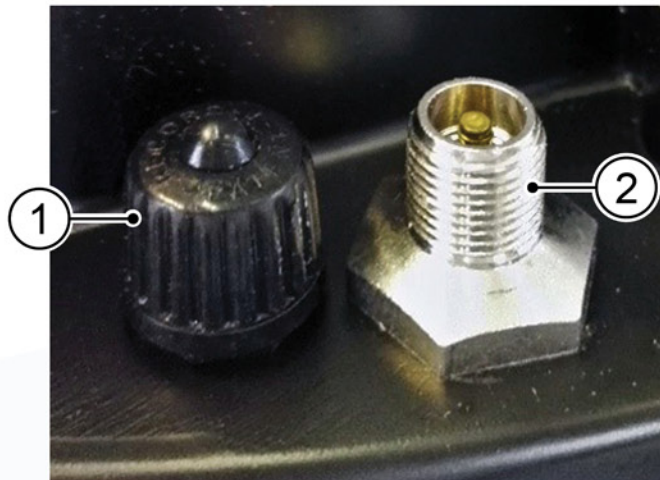
Figure 14 - Lower cover with pressure valve
