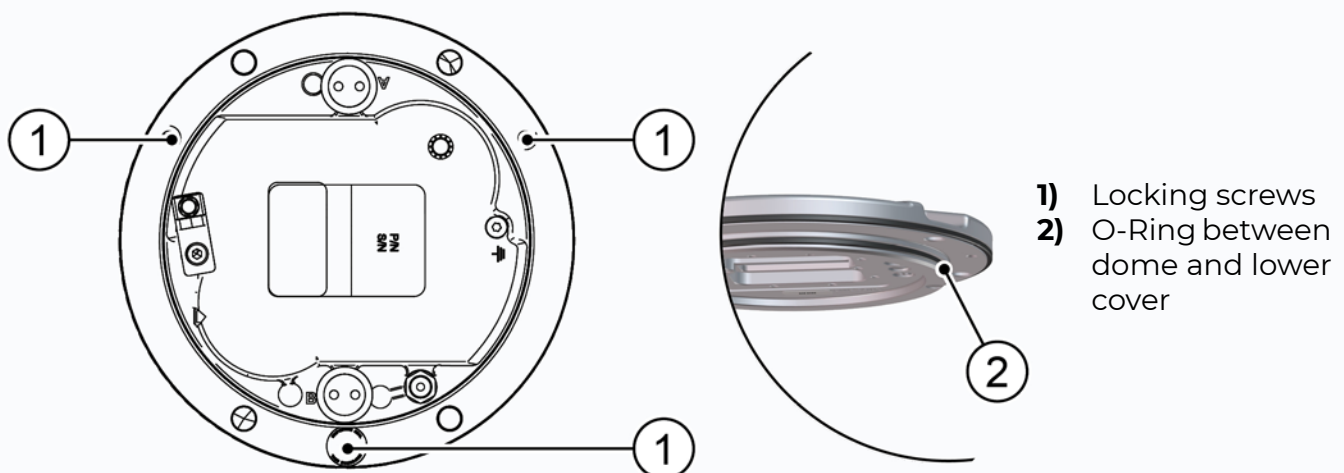
Figure 13 - Lower cover fixing screws
