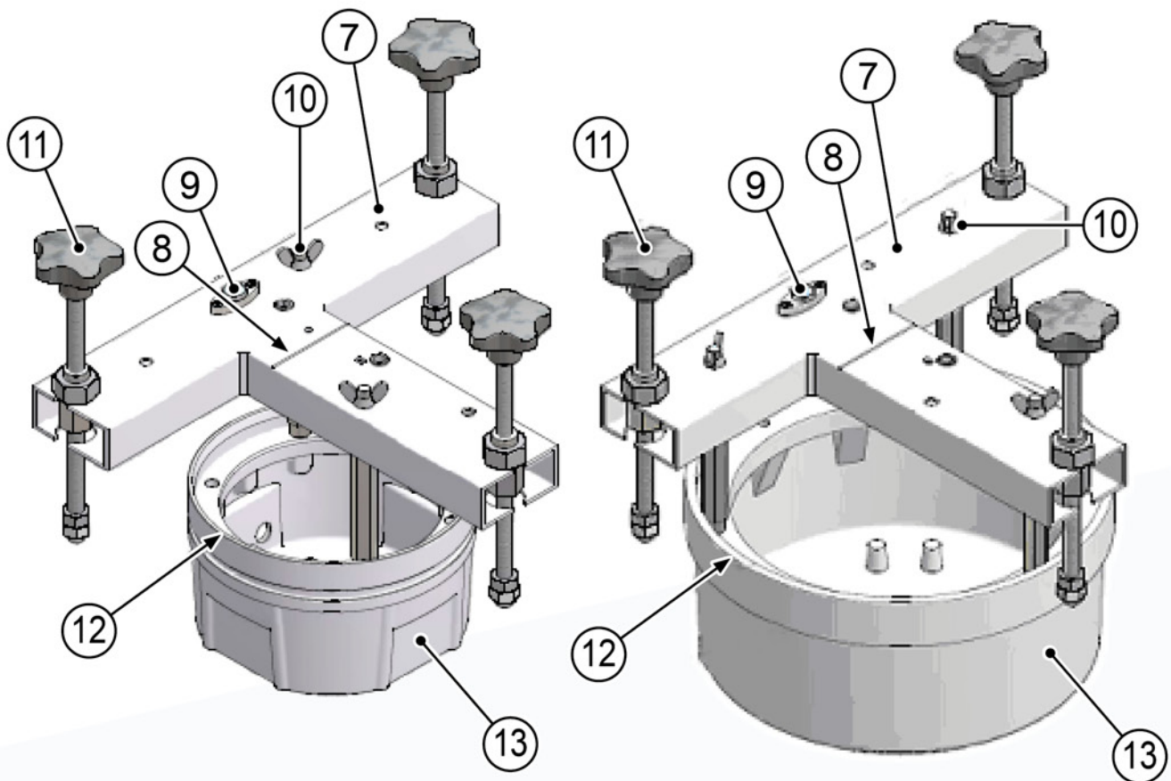
Figure 14 - Shallow base installation details (8" on the left, 12" on the right)
