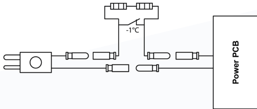
12" Bidirectional Light fixture with 1 power input
