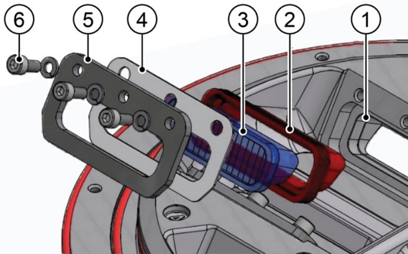
Figure 18 - Prism replacement
