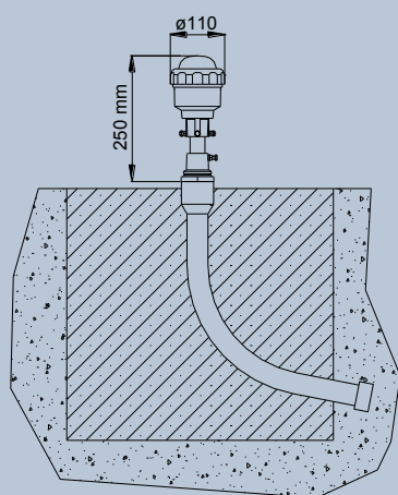
Pipe Elbow
