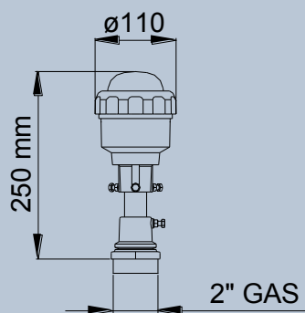
Overall Dimensions
