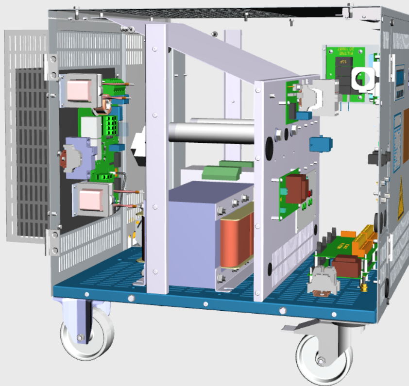
DIAM4200 1 to 2.5 kVA – Internal View
